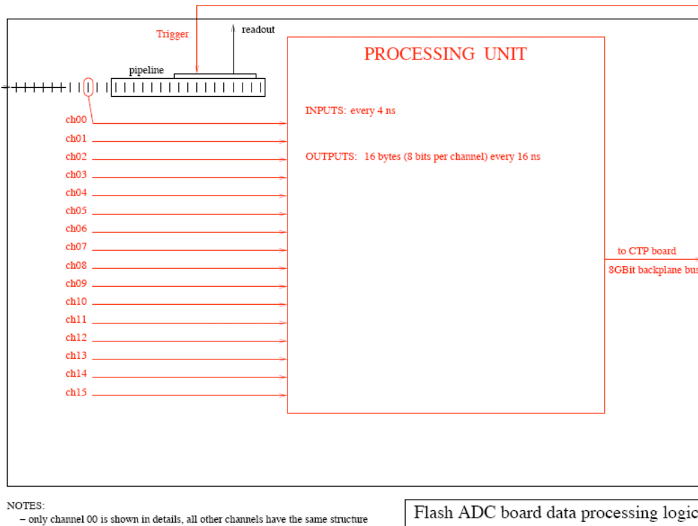
Fig. 4.6.5.1 Processing unit on the FADC board
