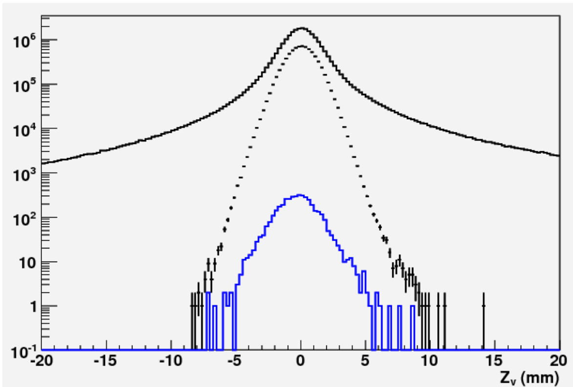
Figure 5.3.2.4: Distribution of the reconstructed vertex position along the beam axis for 6.6GeV 200MeV A' events before (solid black) and after (points with errors) selection. The blue histogram shows the distribution for pairs that have at least one bad hit after selection.
