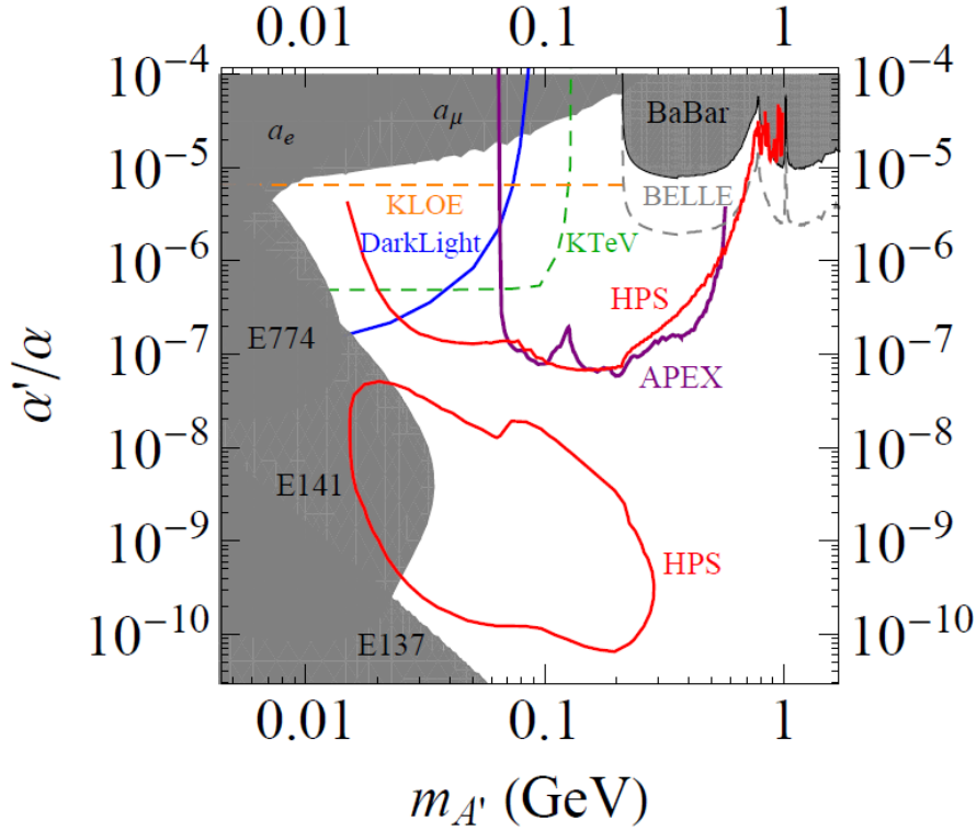
Figure 2.3.1 Anticipated reach in \alpha'/\alpha = \epsilon^2 for the Heavy Photon Search (HPS) experiment at Hall B in JLab (red lines) with existing constraints on an A' from electron and muon anomalous magnetic moment measurements, a_e and a_\mu (see [54]), the BaBar search for Y(3S) \rightarrow \gamma \mu^+ \mu^- [49], and three beam dump experiments, E137, E141, and E774 [55, 56, 57] (see [11]). The a_\mu and Y(3S) limits assume equal-strength couplings to electrons and muons. Also shown are estimates of potential 2\sigma sensitivities for A' searches in existing data (thin dashed lines), assuming optimal sensitivity as described in the text: KTeV \pi^0 \rightarrow \gamma A' \rightarrow \gamma e^+ e^- (green dashed curve), KLOE \Phi \rightarrow \eta A' \rightarrow \eta e^+ e^- (orange dashed curve) and Belle e^+ e^- \rightarrow \gamma A' \rightarrow \gamma \mu^+ \mu^- (gray dashed curve). In addition, we show the projected 2\sigma sensitivities for the proposed “APEX” experiment in JLab Hall A (purple) [58] and the proposed “DarkLight” experiment using the JLab Free-Electron Laser (FEL) (blue) (we show the 5\sigma sensitivity taken from [59]). The HPS lines assume an electron beam with a current of 450 nA (200 nA) incident for 9 \times 10^6 seconds on a 0.25% (0.125%) radiation length tungsten target and a beam energy of 6.6 GeV (2.2 GeV). The upper solid red lines correspond to the 2\sigma sensitivity of a full resonance search. The lower contours denote the sensitivity of a vertex-based resonance search. Here the lines correspond to 2.4 signal events where the vertex requirement was chosen to have 0.5 expected background events in each resolution-limited mass window. The full detector, trigger, and vertexing efficiencies have been included in these estimates. See Section 6 for a more detailed discussion.
