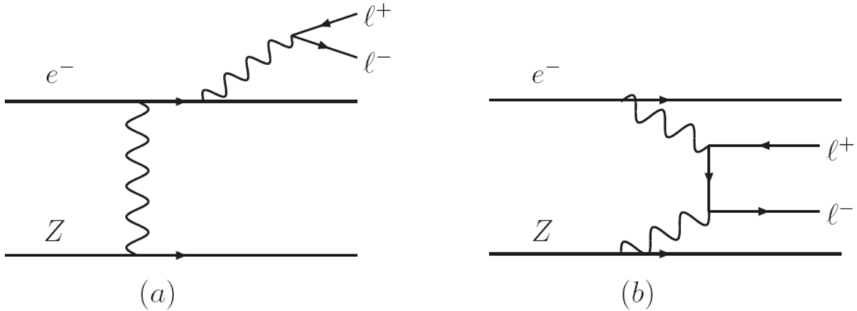
Figure 3.2.1: Sample diagrams of (a) radiative trident ( \gamma^* ) and (b) Bethe-Heitler trident reactions that comprise the primary QED background to A' \rightarrow l+l^- search channels.
